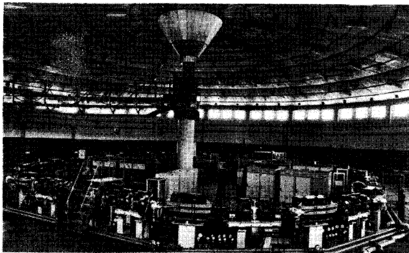
An electron storage ring in China's synchronous radiation laboratory.
